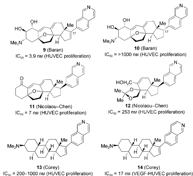
Scheme 3. Selected cortistatin analogues capable of inhibiting proangiogenic endothelial cell behaviors.
